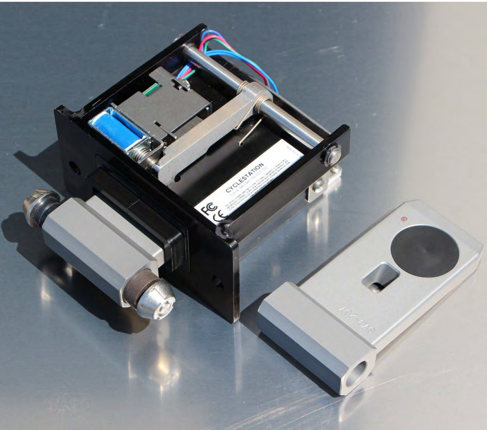
Solar Powered Bike Share Lock
